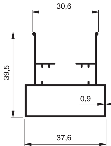
1958 - 0.448 Kg/m
