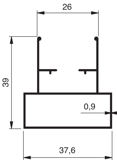
1957 - 0.418 Kg/m
