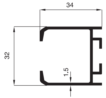
1870 - 0.534 Kg/m
