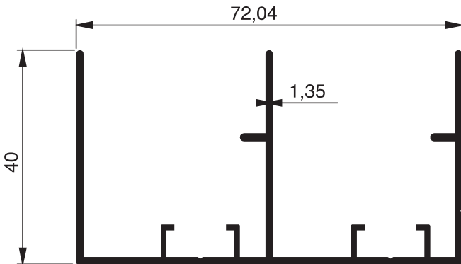
1911 - 0.815 Kg/m
