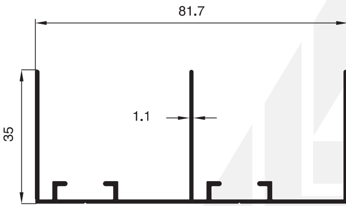
2017 - 0.644 Kg/m
