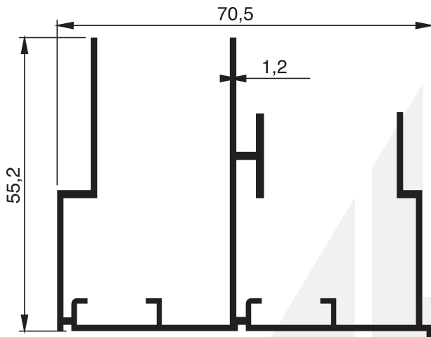
1886 - 0.910 Kg/m
