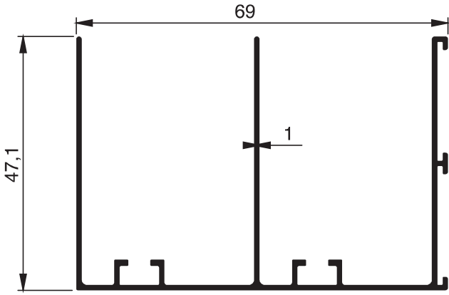
1873 - 0.665 Kg/m
