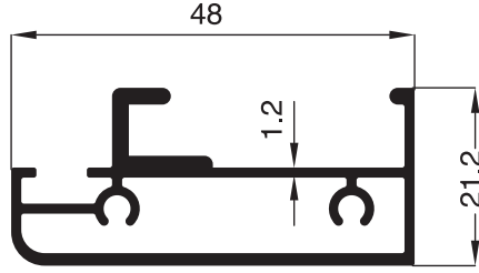
1841 - 0.640 Kg/m
