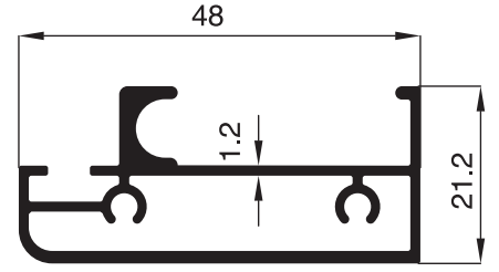
2108 - 0.625 Kg/m
