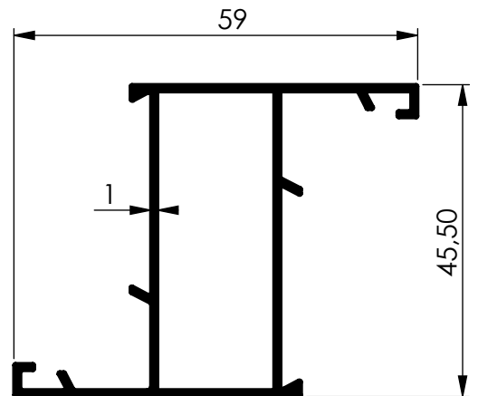
965 0.542 Kg/m
