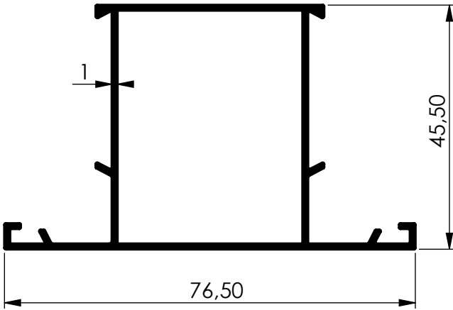
961 0.636 Kg/m
