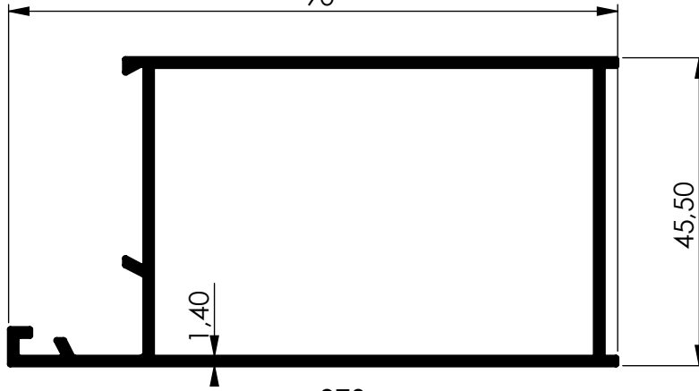
970 0.992 Kg/m
