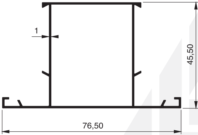
961 - 0.636 Kg/m
